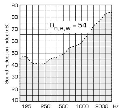
Fresh 80-dB with 400mm wall pipe.
